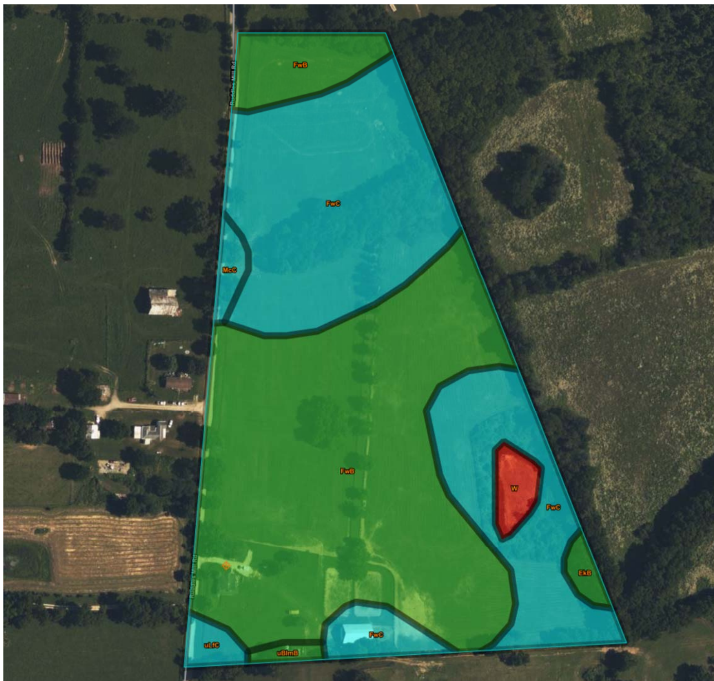
Summary by Map Unit — Bourbon and Nicholas Counties, Kentucky (KY604)
